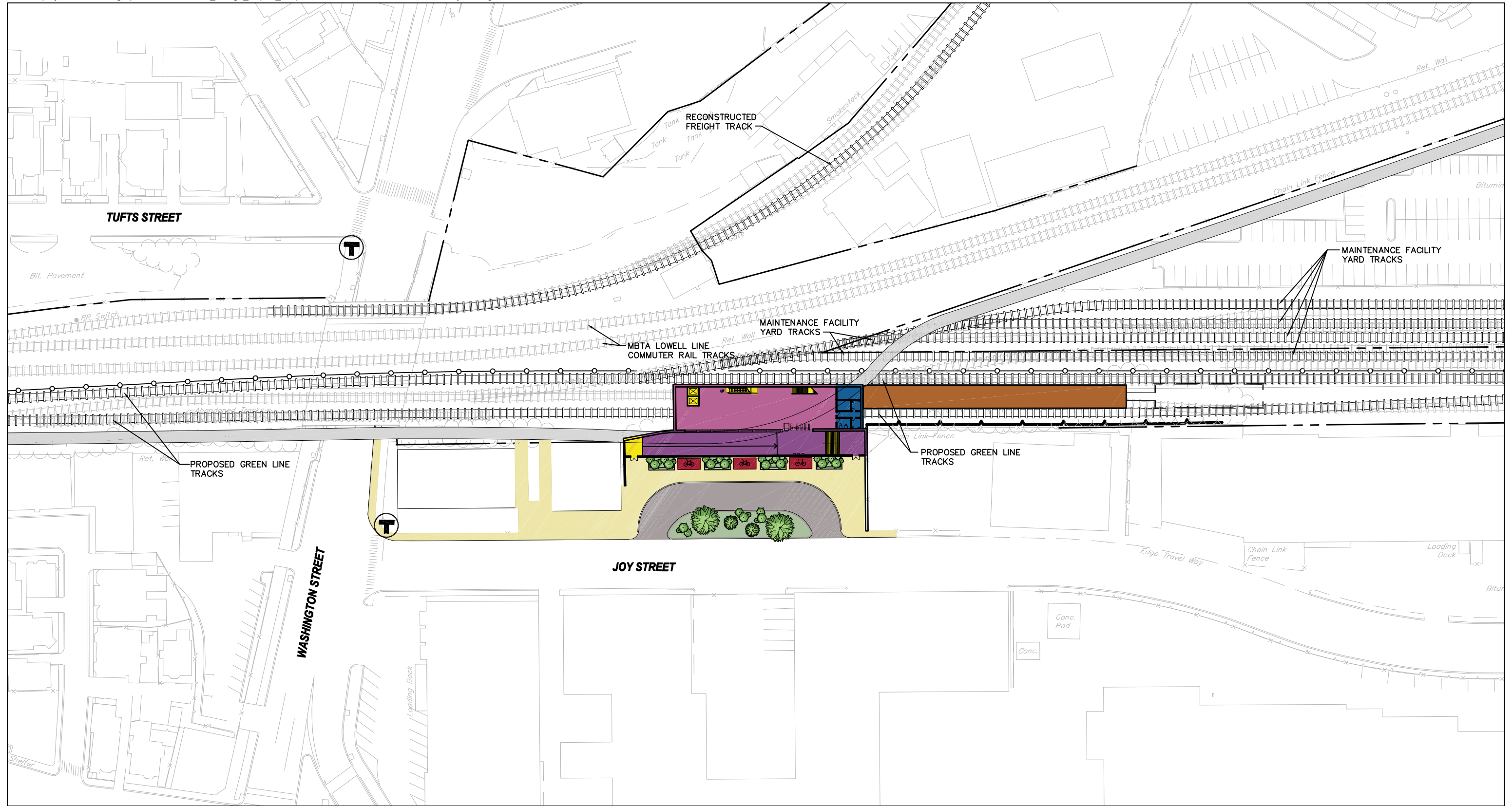
Figure 3.7-6 Brickbottom Station Station Layout
