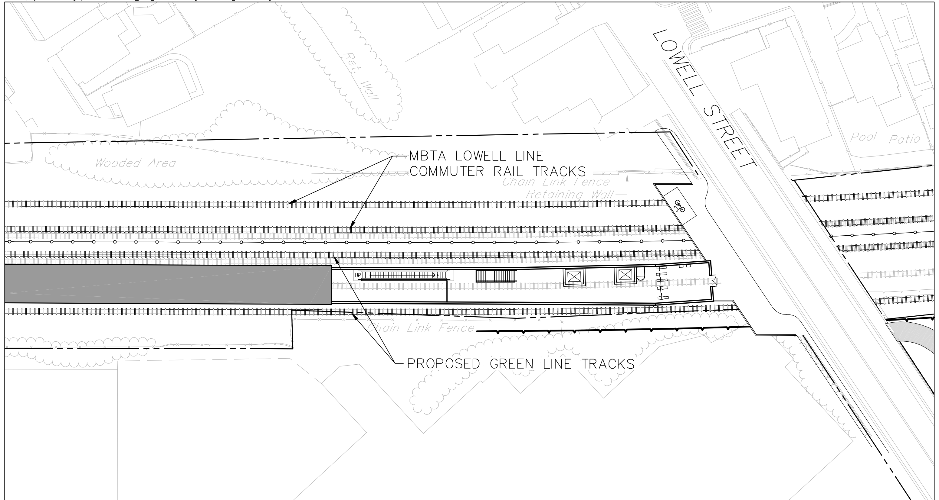
Figure 3.7-15 Lowell Street Station Station Plan
