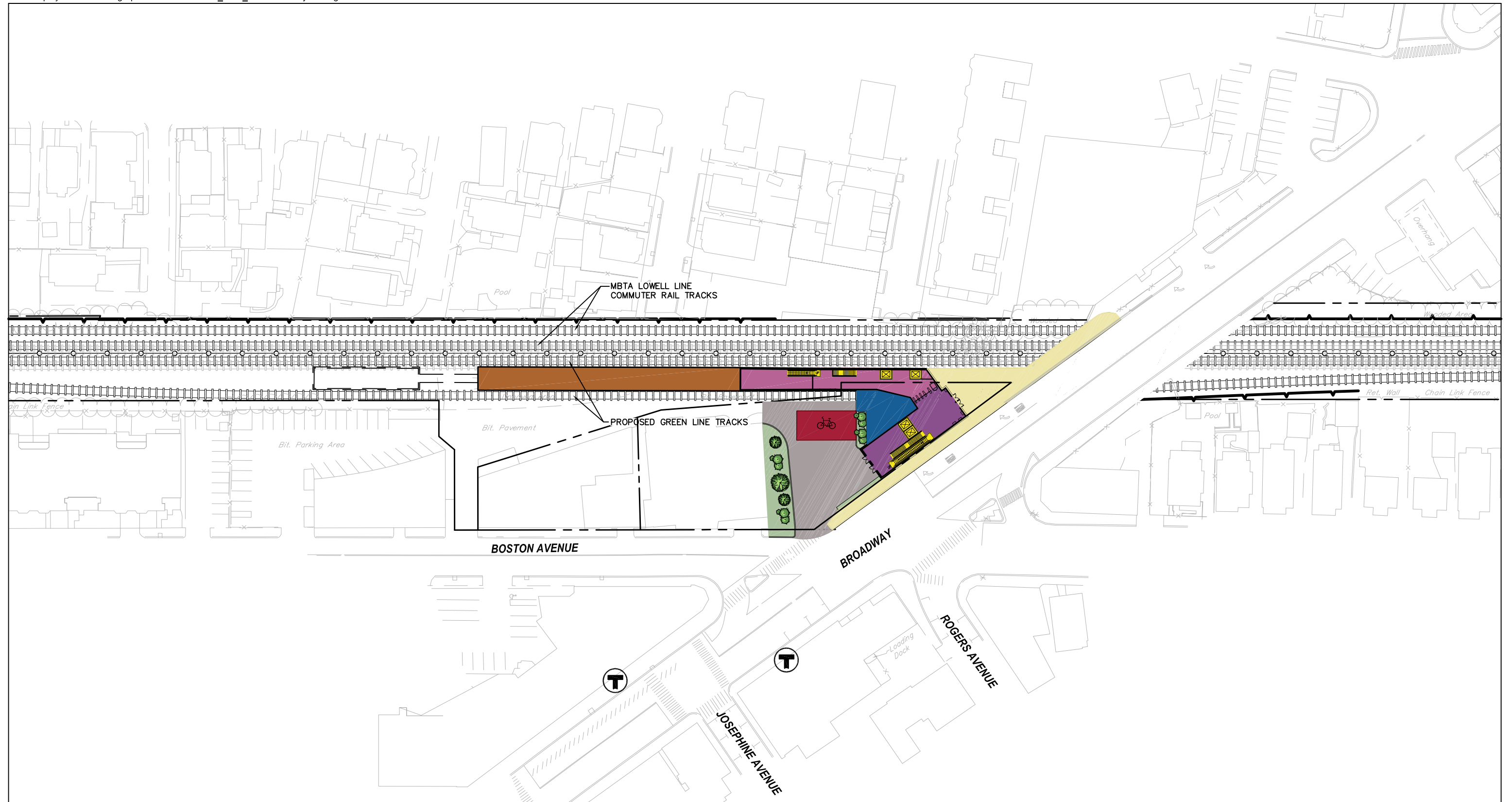
Figure 3.7-18 Ball Square Station Station Layout
