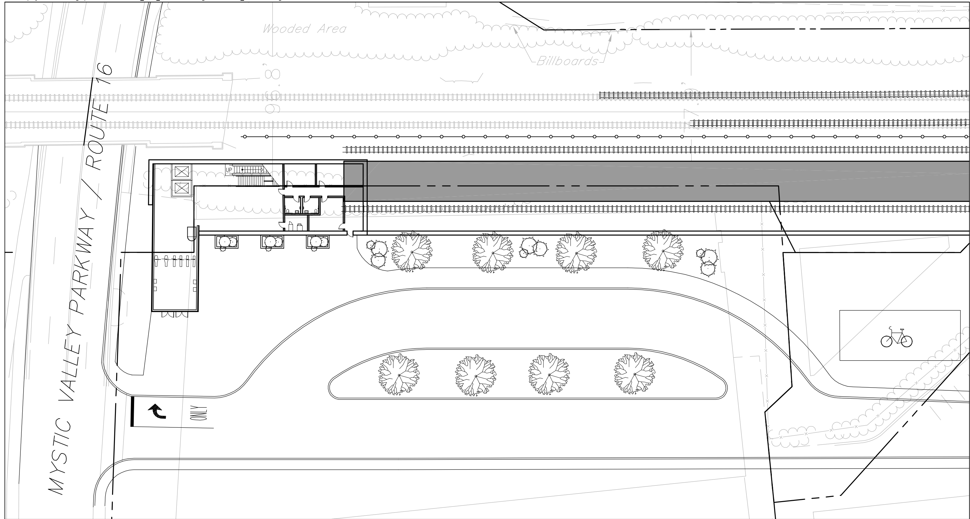
Figure 3.7-28 Mystic Valley Parkway / Route 16 Station Station Plan
